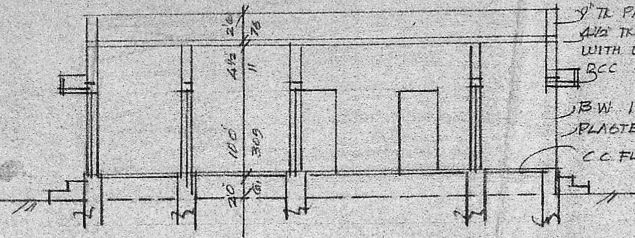
SECTION AA
