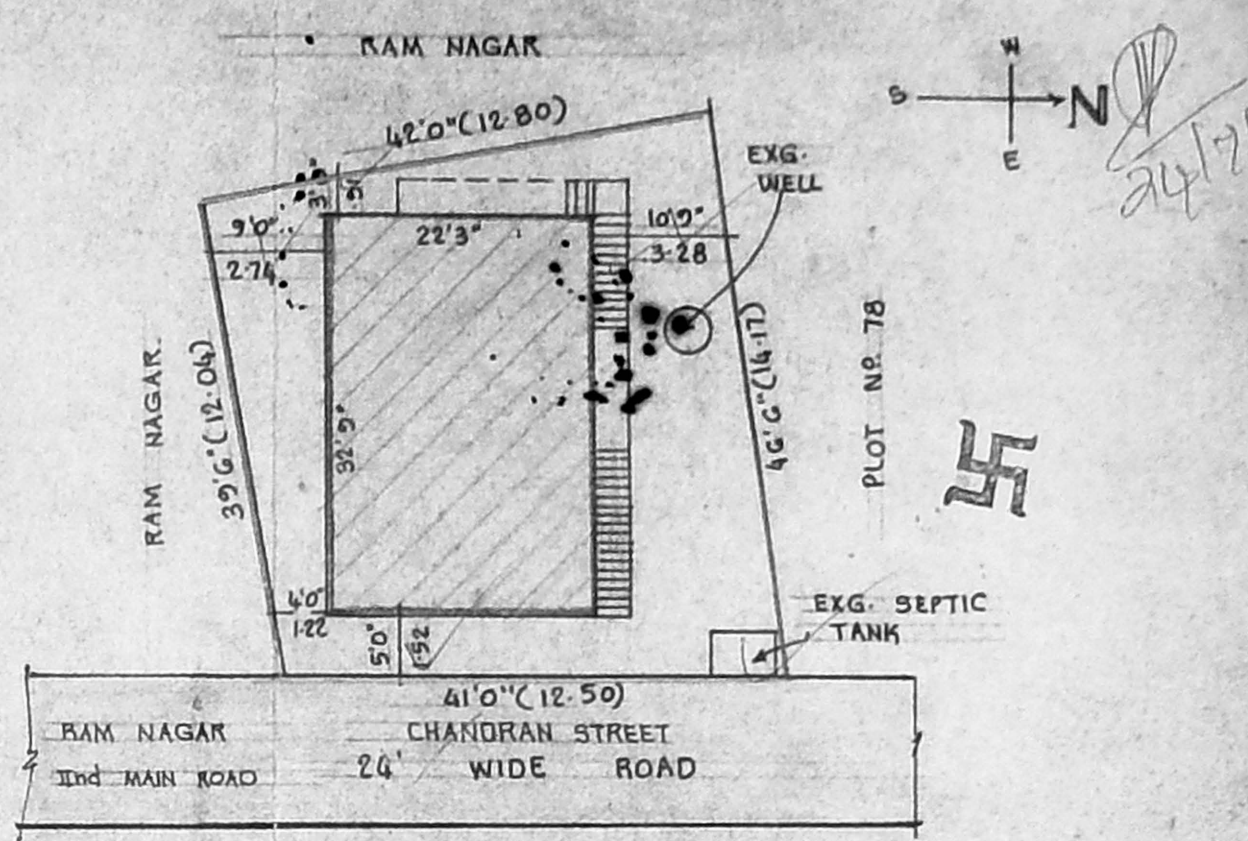
SITE PLAN
